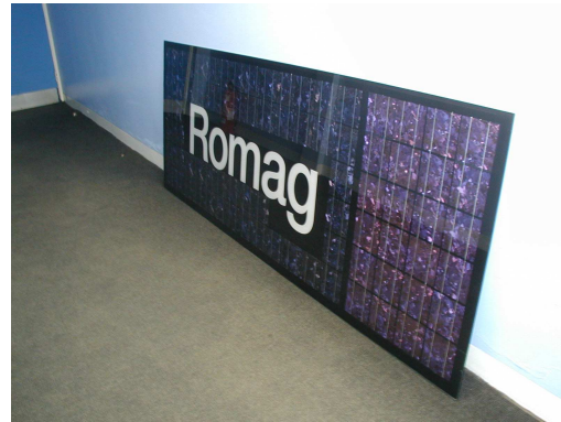
Figure 7 - Two colour 72 cell Romag module
