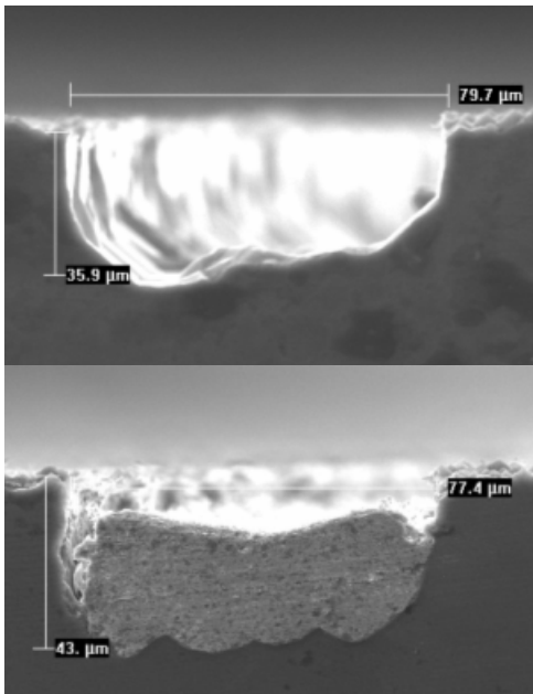
Figure 2. Laser formed groove ‘finger’ before and after screen printing.
