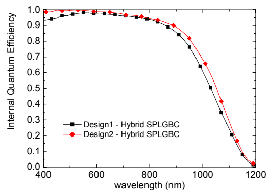
Figure 3. Internal Quantum Efficiency comparison of Design1 and Design2 screen printed cells
