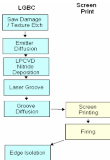
Figure 1. The hybrid process designed to produce SPBCSCs.
